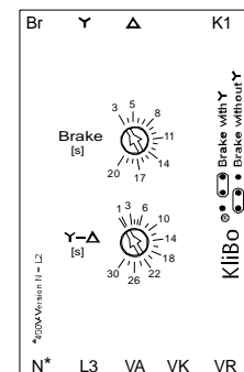
Bedienfeld KLIBO-Phase-Brake
